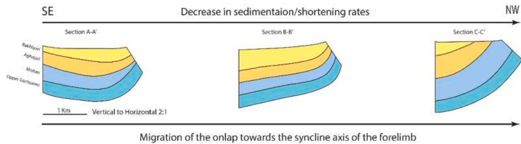
Fig. 12. Migration of pinch-out in the growth strata layers along the Mansourabad anticline related to the southwestern syncline. Locations are shown in Figs. 4, 6 and 7.
