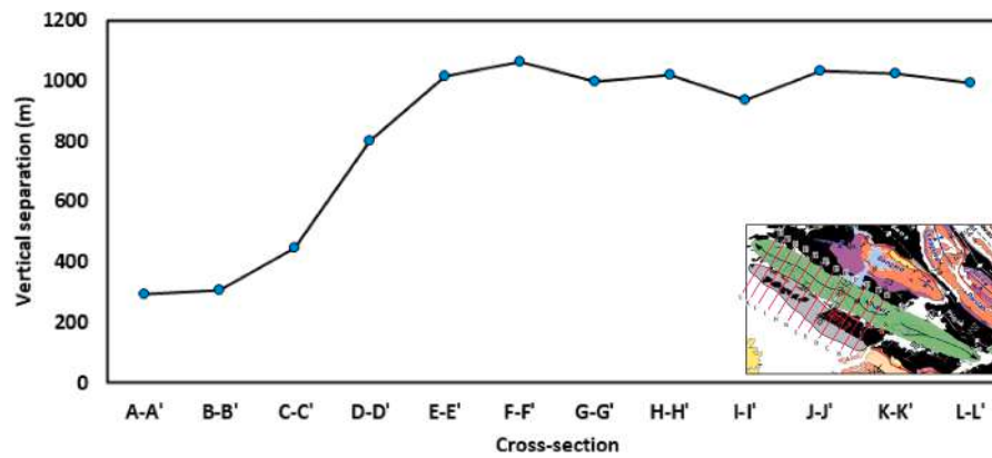
Fig. 10. Vertical separation profile of forelimb Behbahan thrust fault along the Mansourabad anticline for the Asmari Formation. The inset illustrates location of the cross-sections (also see Fig. 3 for more details).
