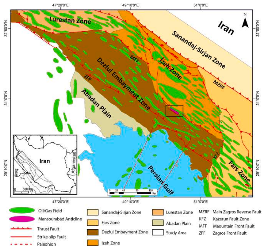
Fig. 1. The structural map of the ZFTB shows tectono-stratigraphic subdivisions (modified after Fard et al., 2006). The Mansourabad anticline is marked in pink at the northern boundary of the Dezful Embayment.
