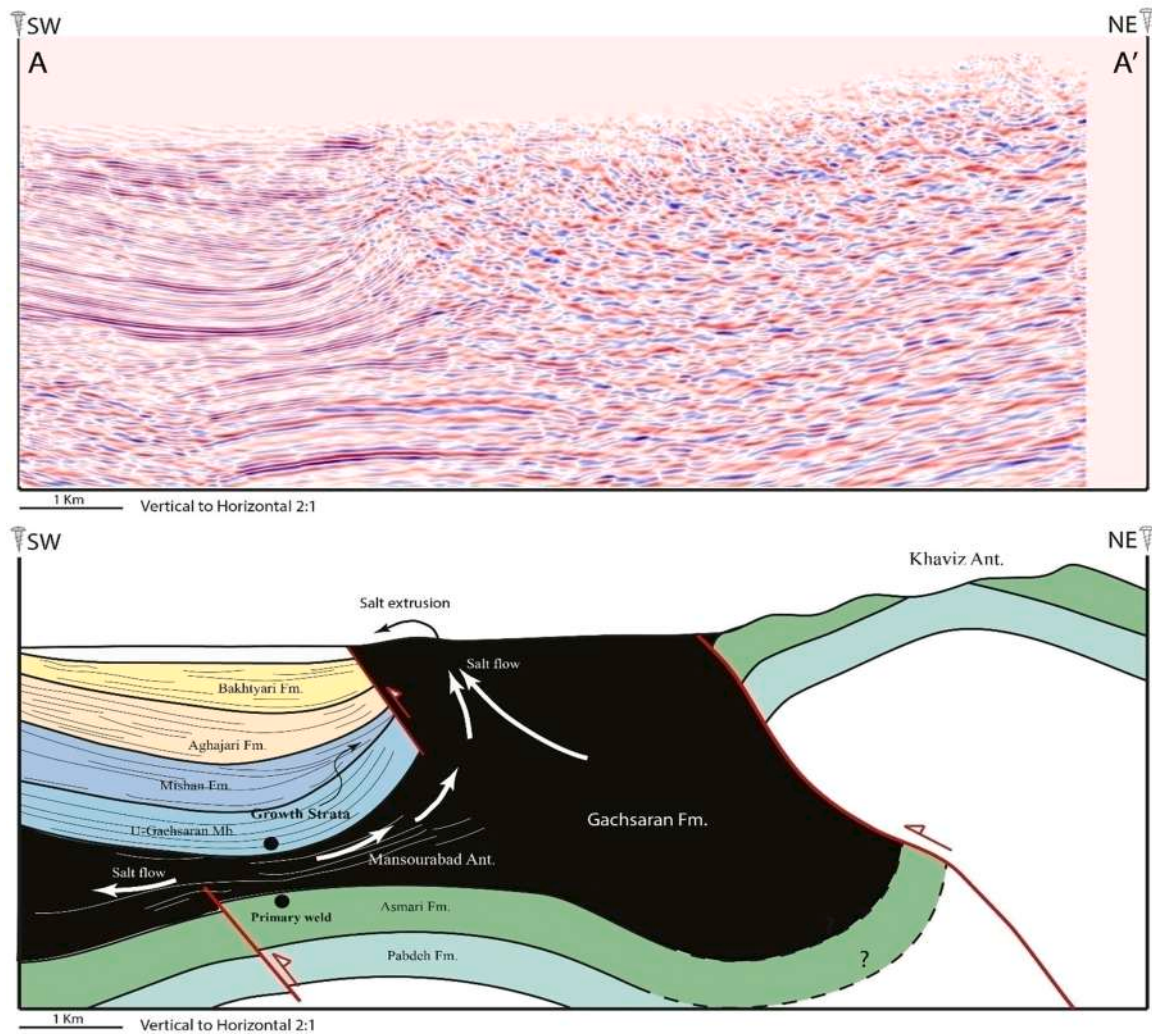
Fig. 4. Uninterpreted (upper) and interpreted (lower) seismic profile through the SE plunge of the Mansourabad anticline. Fig. 3 presents the location of the profile. In this profile, the Mansourabad anticline is a gentle detachment fold with NE-verging. The right side of the image is extrapolated from surface data e.g., Heydarzadeh et al. (2021).
