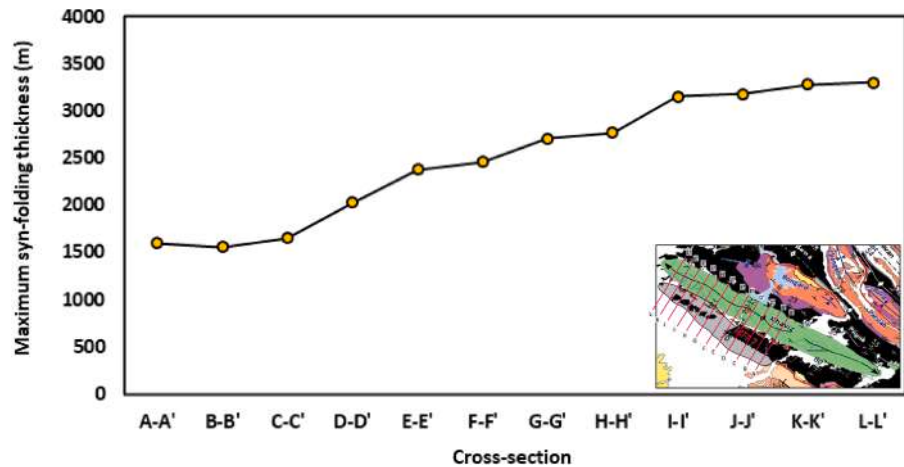
Fig. 13. Maximum thickness of syn-folding strata (Mishan, Aghajari, and Bakhtyari Formations) along the Mansourabad anticline. The inset illustrates location of the cross-sections (also see Fig. 3 for more details).
