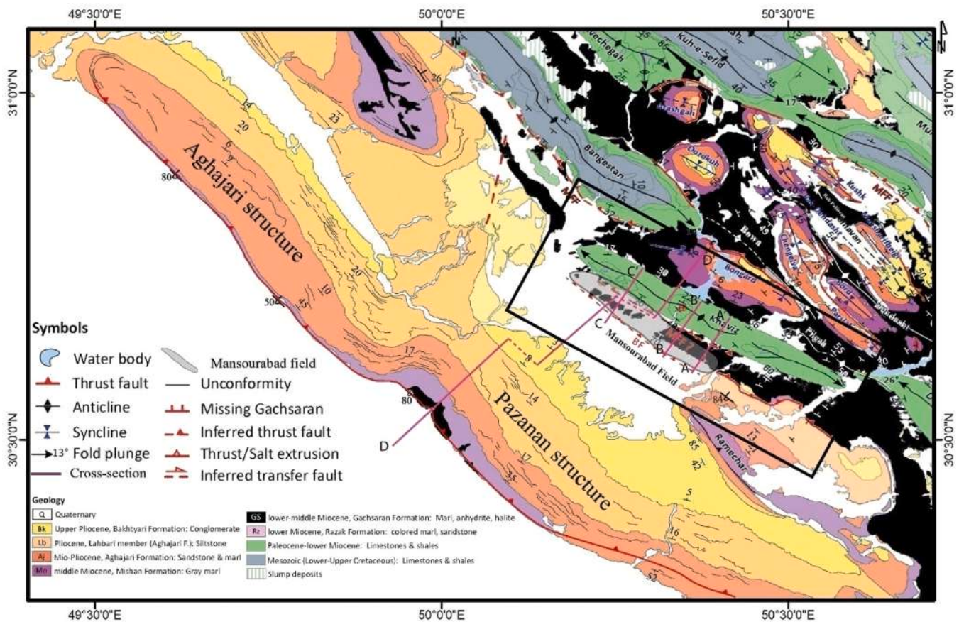
Fig. 3. Geologic map of the study area. Locations of the studied anticline (Mansourabad and Khaviz anticlines) are shown by the gray polygon. (modified after Najafi and Lajmork, 2020; Heydarzadeh et al. 2021). The MFF and BF refer to the Mountain Front Fault and Behbahan Fault, respectively.
