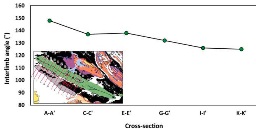
Fig. 15. Interlimb angle of the Mansourabad anticline in different selected seismic profiles.
