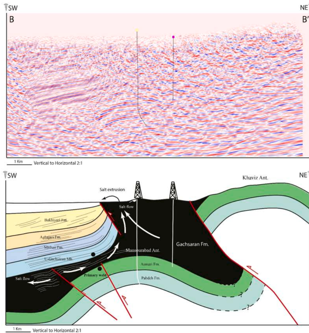
Fig. 6. Uninterpreted (upper) and interpreted (lower) seismic profile through the near the central part of the Mansourabad anticline. Fig. 3 for location. Mansourabad anticline appears slightly symmetric. The right side of the image is extrapolated not from the seismic image but from some surface data (e.g., Heydarzadeh et al. 2021).
