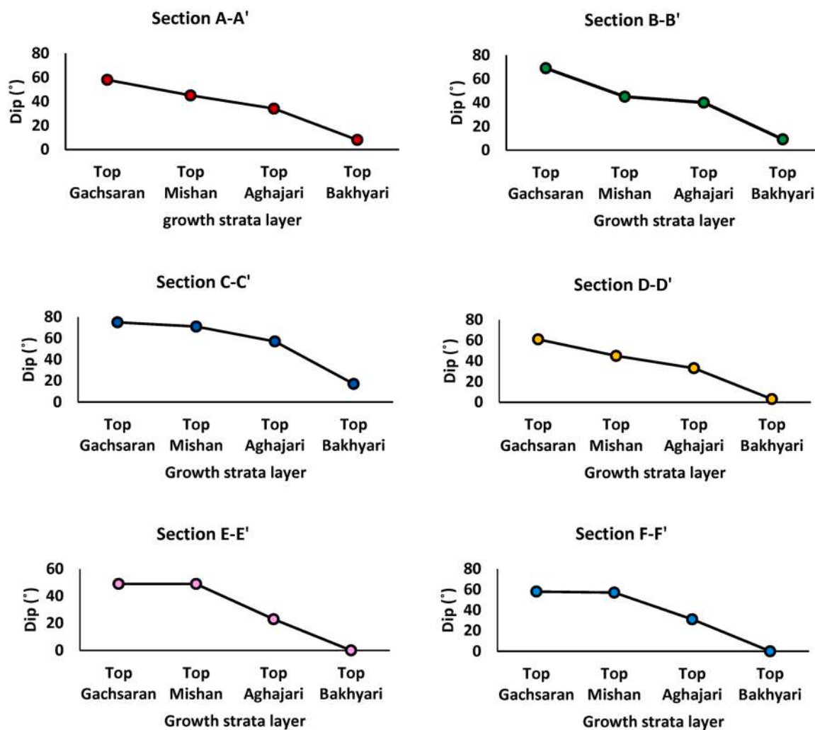
Fig. 11. Variations of the dip of growth strata layers in different selected seismic profiles at the junction with the Behbahan Fault (Figs. 4–8).
