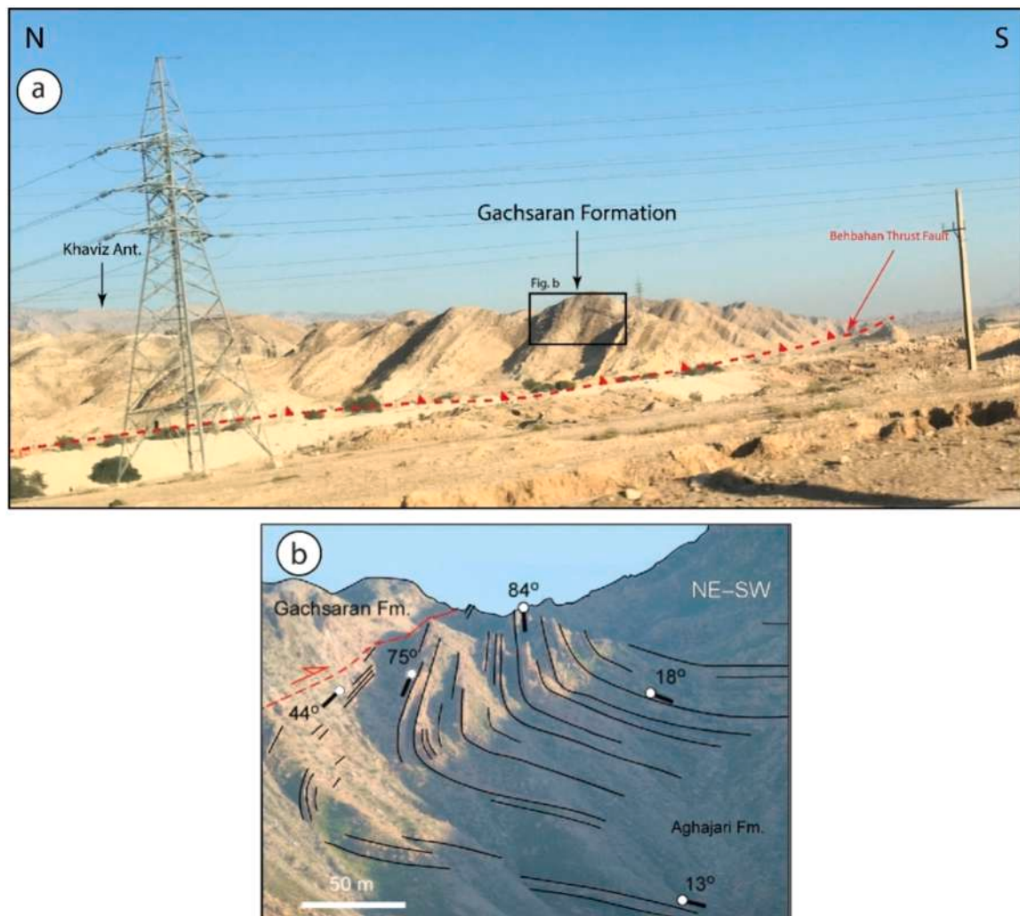
Fig. 5. a,b. Effect of Behbahan thrust fault in the Gachsaran Formation, which thrust over the Aghajari Formation at the southern flank of the subsurface Mansourabad anticline, (the inset b is from Najafi and Lajmorak, 2020).
