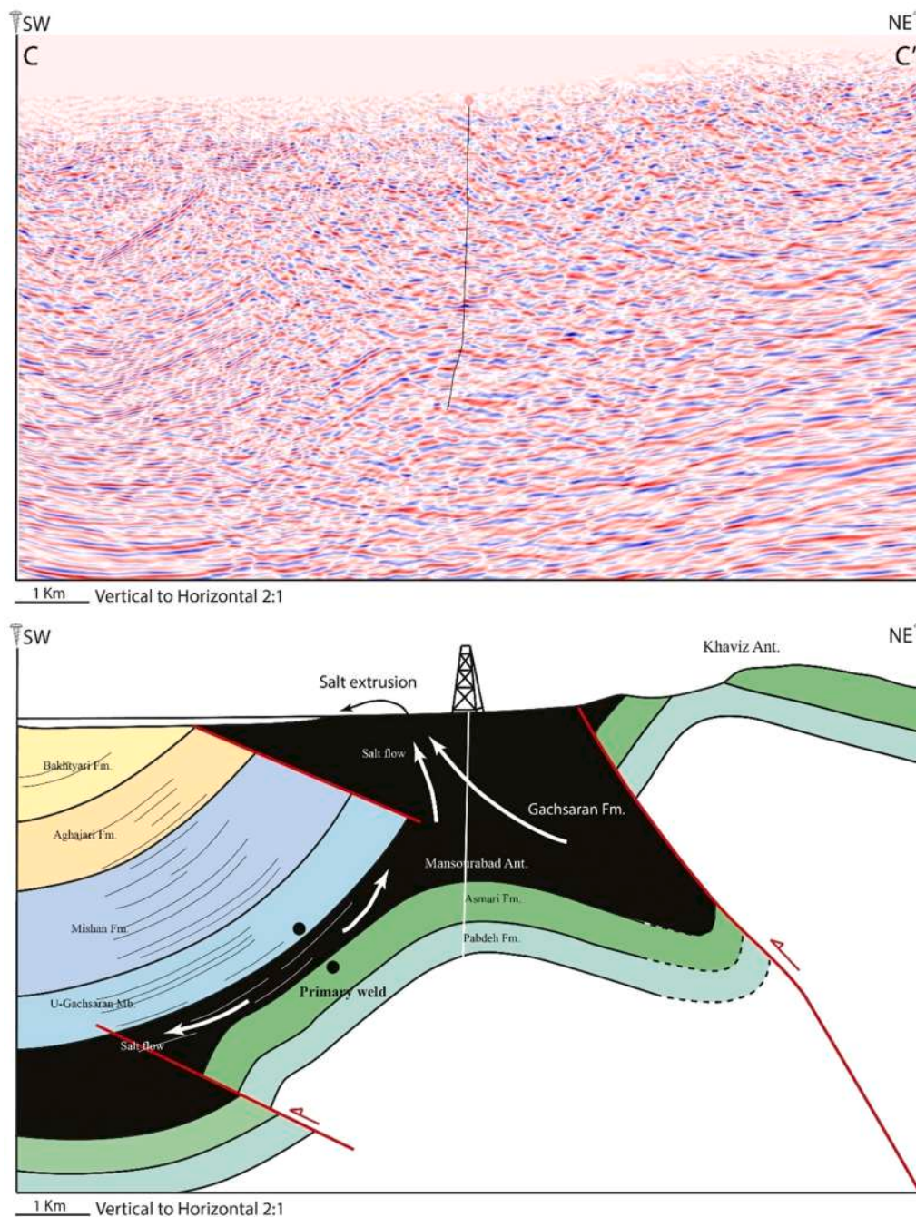
Fig. 7. Uninterpreted (upper) and interpreted (lower) seismic profile through the NW part of the Mansourabad anticline. Fig. 3 for location. The right side of the image is extrapolated from surface data e.g., Heydarzadeh et al. (2021).
