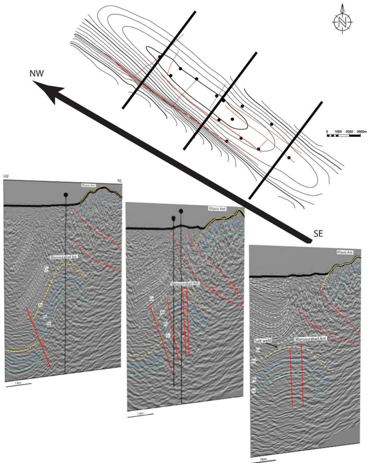
Fig. 14. Variations of structural style along the Mansourabad anticline from detachment fold in the southeastern part to fault propagation fold in the northwestern part. Black dots- wells; red lines- faults.
