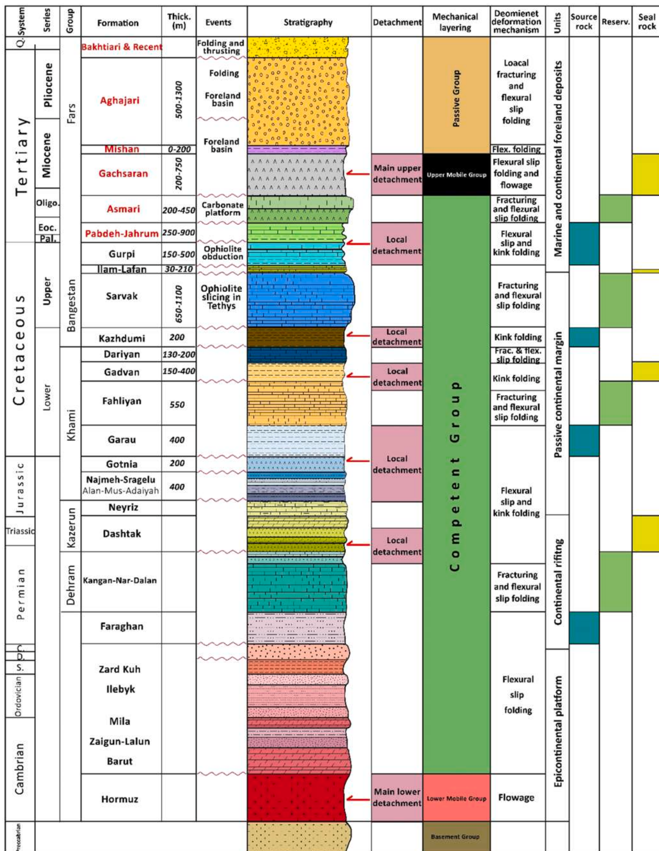
Fig. 2. Lithostratigraphic column of the study area, also shows mechanical zones, detachment units and tectonic events (Modified after Fard et al. 2006; Bordenave and Heger, 2010). Units in the study area (as seen in the black rectangle in Fig. 3) are stated in red.
