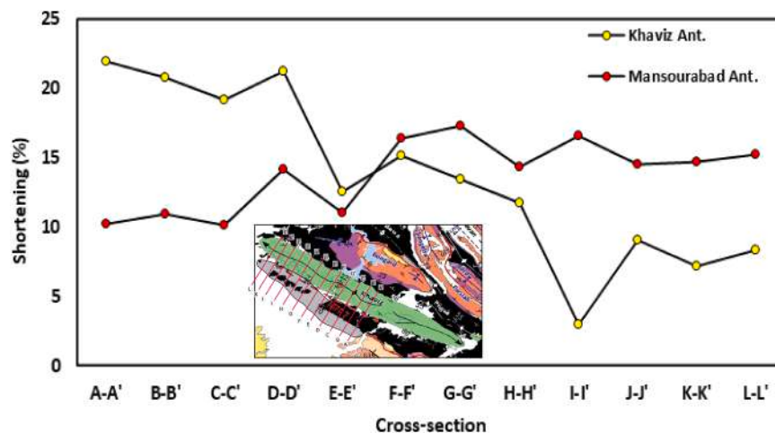
Fig. 9. Along-strike shortening percentage of the Mansourabad and Khaviz anticlines. The inset illustrates location of the cross-sections (also see Fig. 3 for more details).
