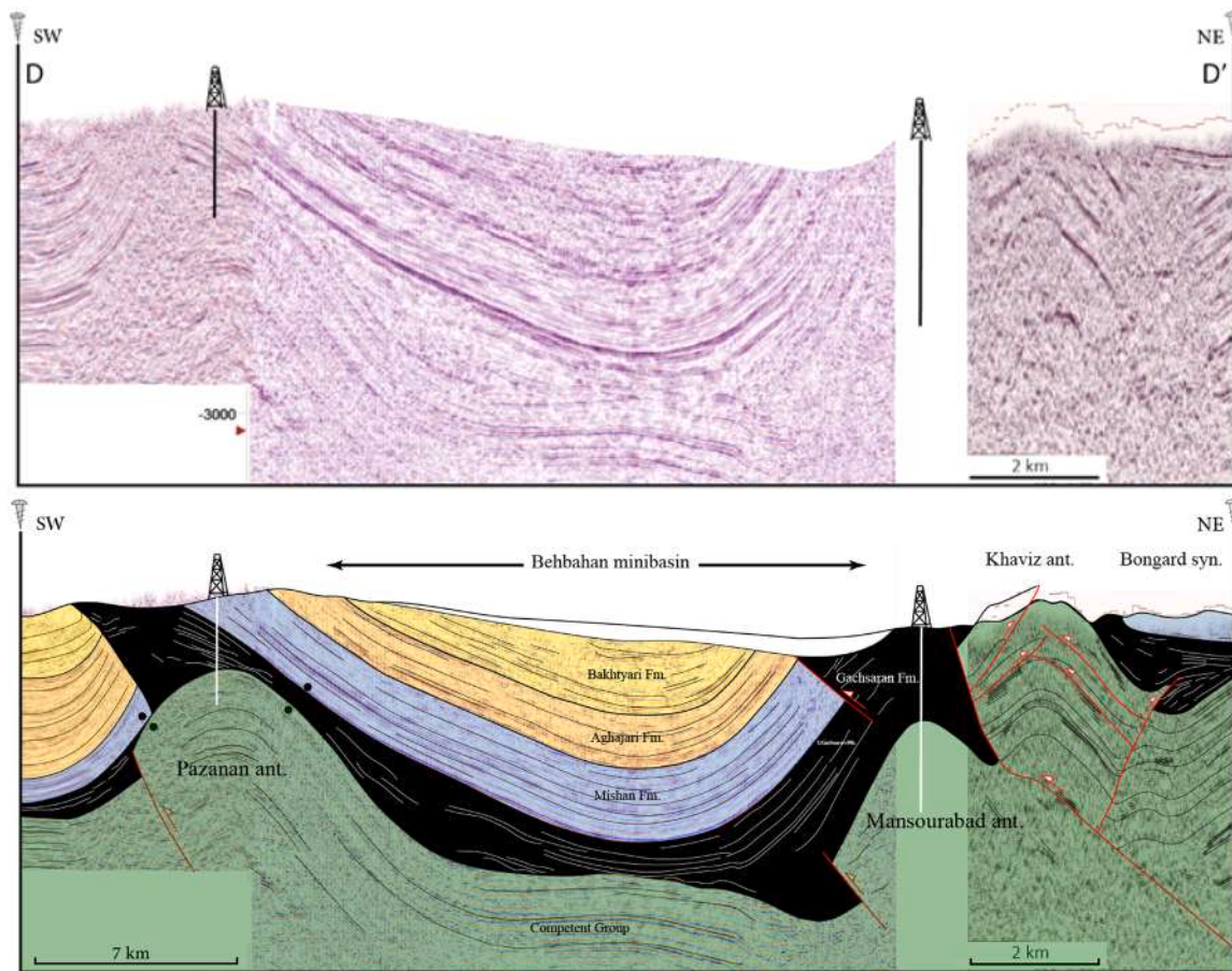
Fig. 8. Uninterpreted and interpreted NE-SW-oriented time-migrated seismic line across the Khaviz, Mansourabad and Pazanan structures. Fig. 3 for location. See also Heydarzadeh et al. (2021).
