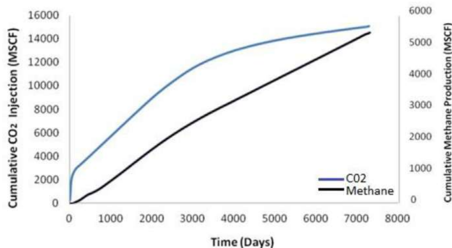
Fig. 10. CO 2 injection over the simulation period and CBM production during the same period. Modified from Vishal et al. (2012).
