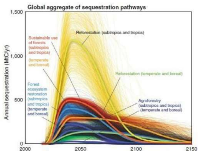
Fig. 4. Terrestrial sequestration pathways showing mean annual sequestration rates from 2000–2150 (reproduced from Meinshausen and Dooley, 2019).
